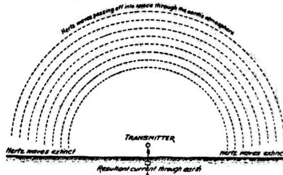
Fig. 13. Diagram Exposing the Fallacy of the Gilding Wave Theory as Propounded In Wireless Text Books.
